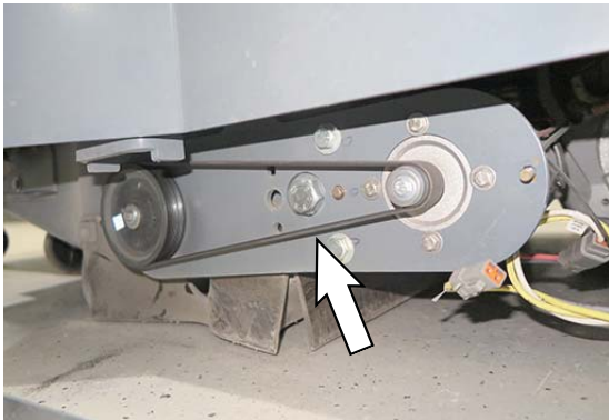
Direct Throw Sweeping Drive Belt (Option)
